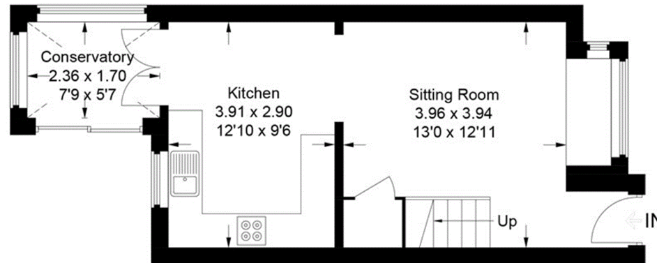
Ground Floor
