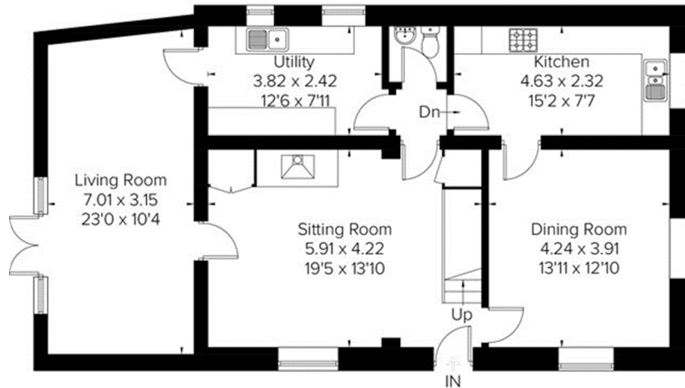
Ground Floor Area = 94.9 sq m / 1021 sq ft (Limited Use Area = 2.3 sq m / 25 sq ft)
