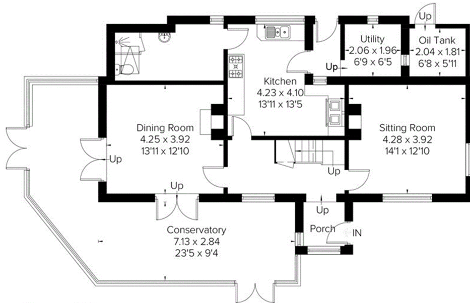
Ground Floor Area = 118.3 sq m / 1273 sq ft (Limited Use Area = 4.8 sq m / 52 sq ft)
