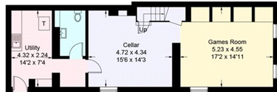
Basement
