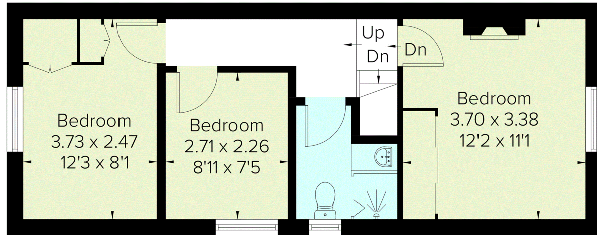
First Floor
