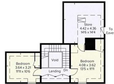
Second Floor Area = 57.3 sq m / 617 sq ft (Excluding Void) (Limited Use Area = 19 sq m / 204 sq ft)
