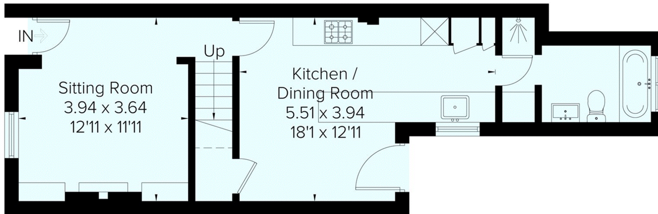
Ground Floor
