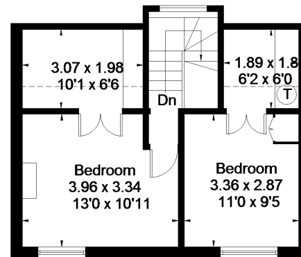
First Floor Area = 39.3 sq m / 423 sq ft (Limited Use Area = 7.2 sq m / 77 sq ft)
