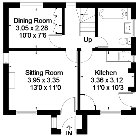
Ground Floor Area = 43.1 sq m / 464 sq ft (Limited Use Area = 0.6 sq m / 6 sq ft)
