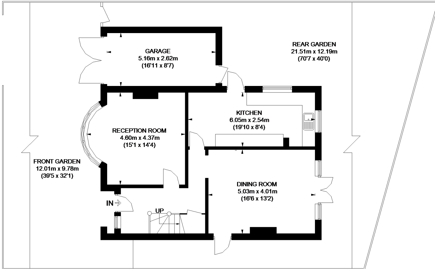
GROUND FLOOR
