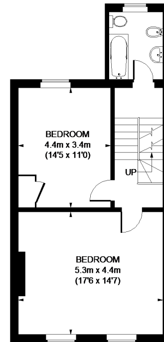
RAISED SECOND FLOOR
