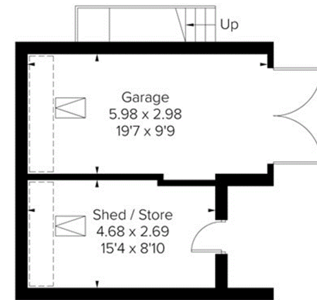
Car Barn Ground Floor
