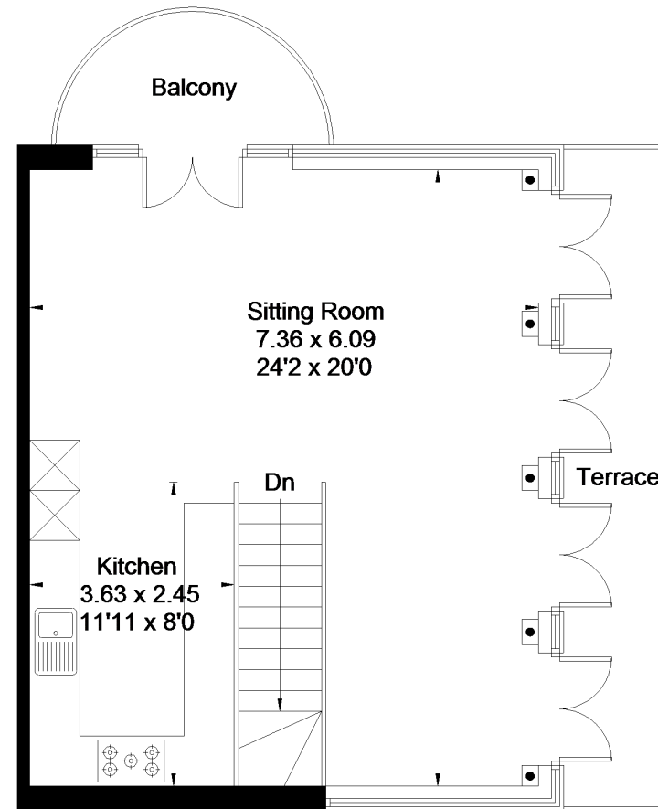
Sixth Floor
