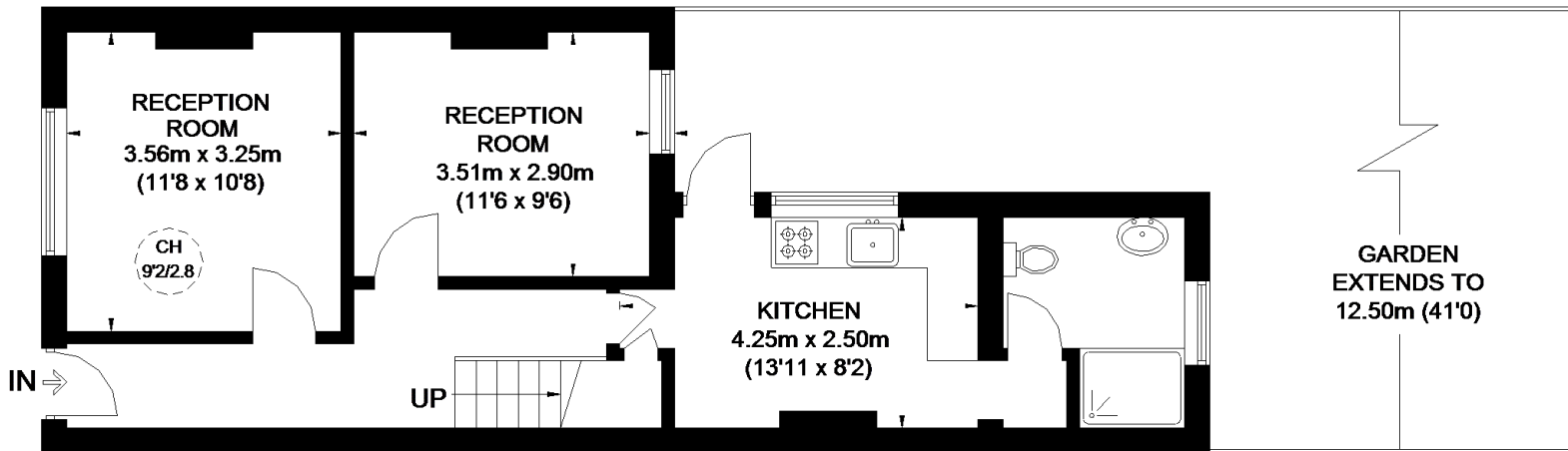
GROUND FLOOR
