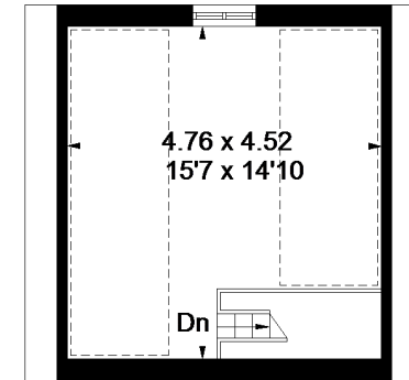
Outbuilding First Floor Area = 21.3 sq m / 229 sq ft (Limited Use Area = 12.3 sq m / 132 sq ft)
