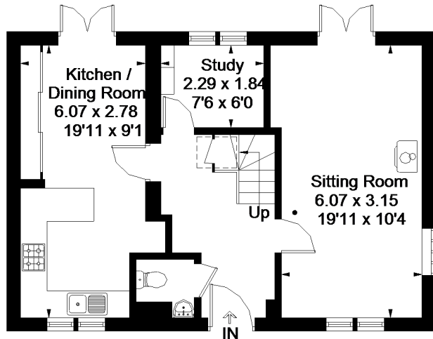
Ground Floor Area = 55.8 sq m / 600 sq ft (Limited Use Area = 0.9 sq m / 9 sq ft)
