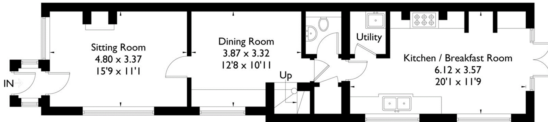
Ground Floor
