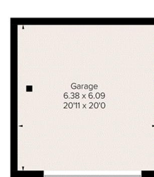
Outbuilding Ground Floor Area = 38.8 sq m / 418 sq ft (Not Shown In Actual Location / Orientation)
