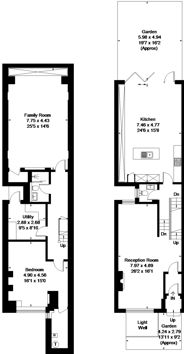
Lower Ground Floor Area = 84 sq m / 904 sq ft (Limited Use Area = 0.6 sq m / 6 sq ft)
