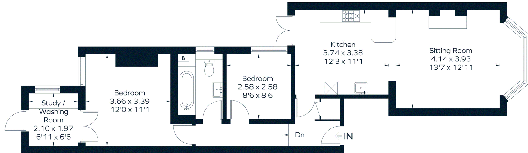
Ground Floor
