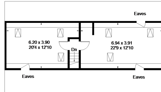
Second Floor
