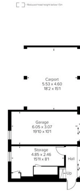
(Not Shown in Actual Location / Orientation) Garage Ground Floor
