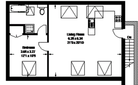
(Not Shown to Actual Location Orientation) Outbuilding - First Floor
