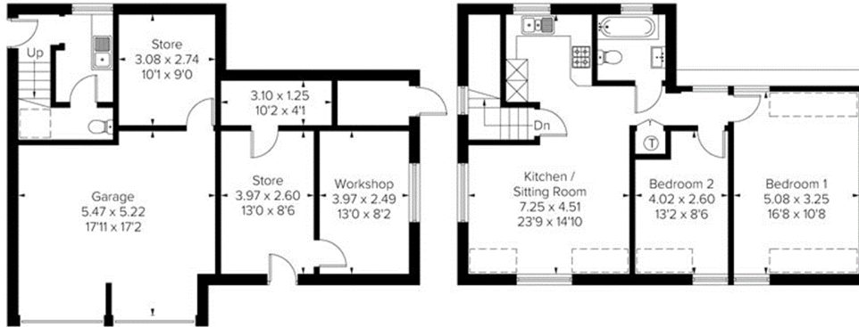
Annexe Ground Floor Area = 74.8 sq m / 805 sq ft (Not Shown In Actual Location / Orientation)
