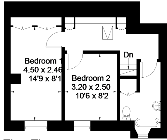
First Floor Area = 34.6 sq m / 372 sq ft
